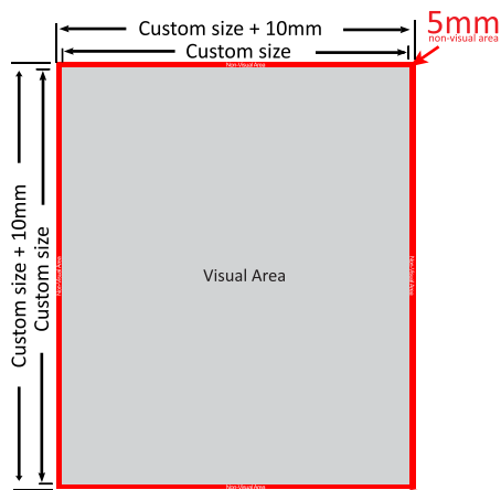
Model Single-sided mounting
