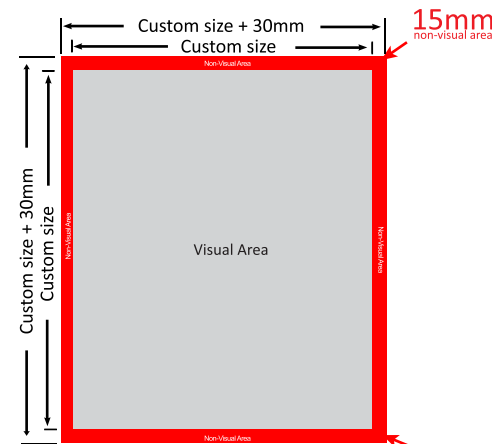
Model Double-sided mounting
