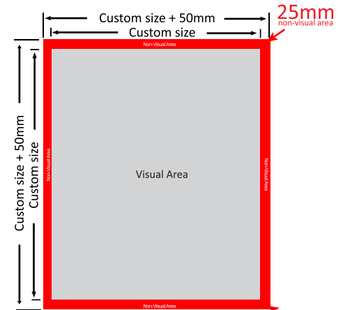
Model Mounting with wrap edges
